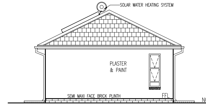
WEST ELEVATION - 1:100
