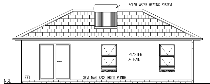
NORTH ELEVATION - 1:100
