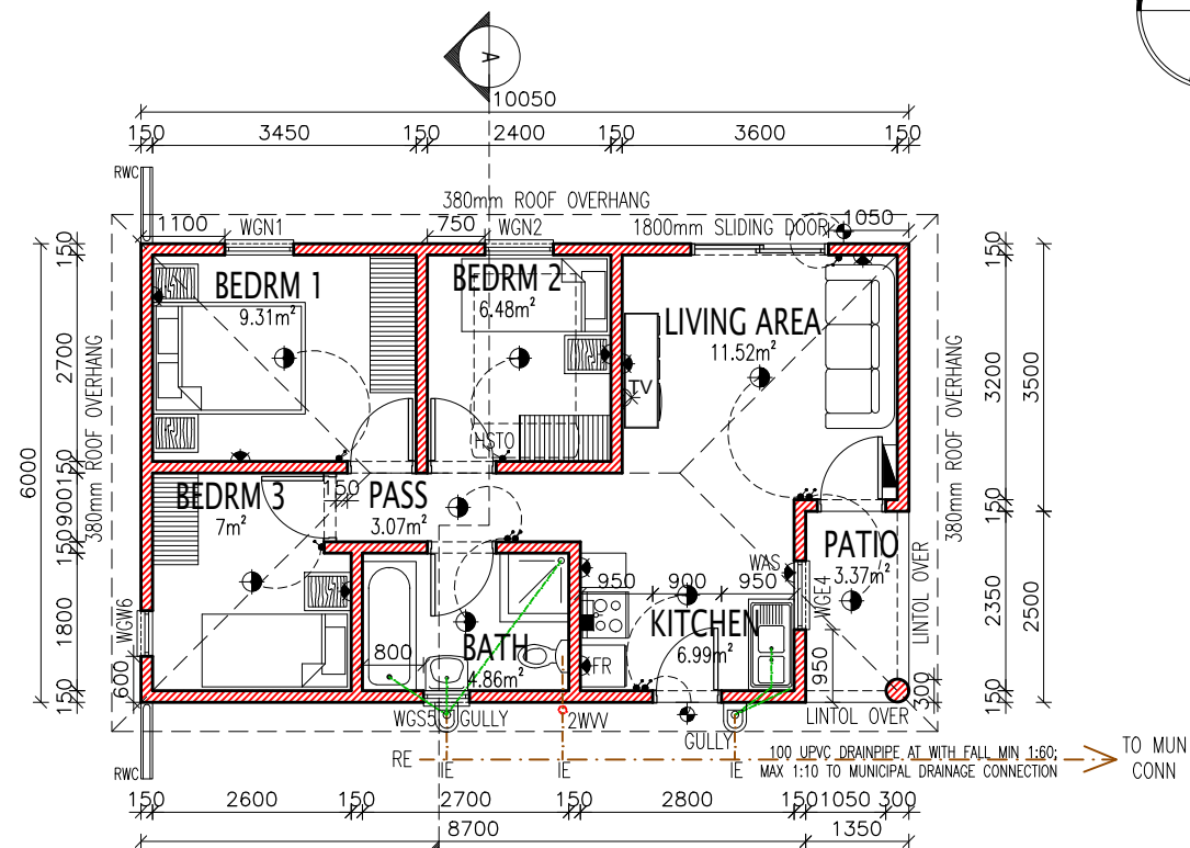
GROUND STOREY - 1:100
