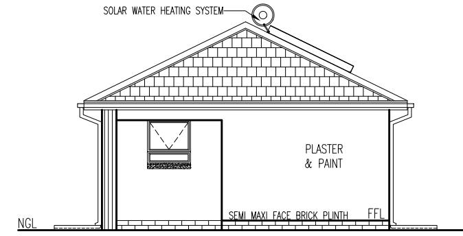
EAST ELEVATION - 1:100
