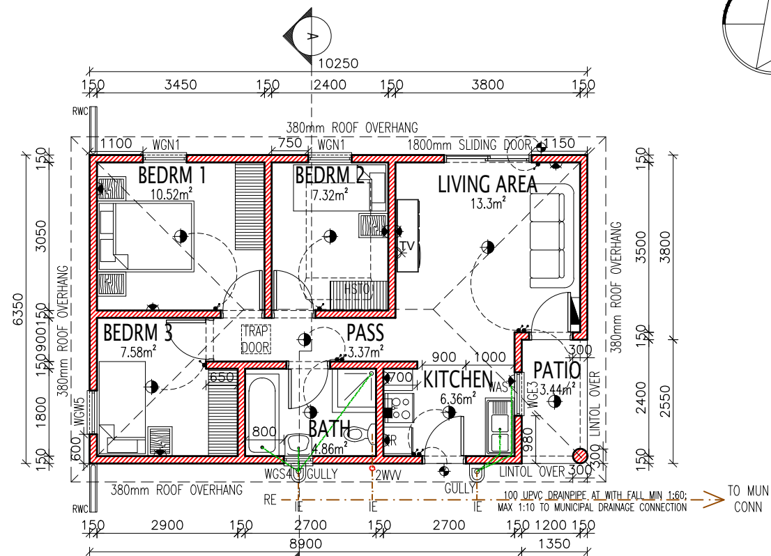
GROUND STOREY - 1:100
