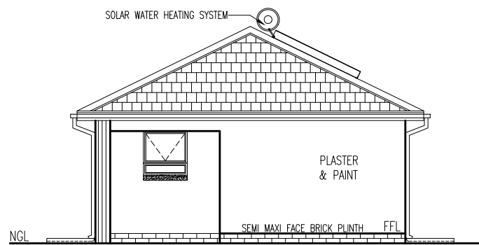
EAST ELEVATION - 1:100
