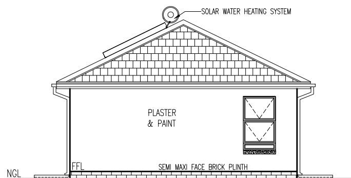
WEST ELEVATION - 1:100
