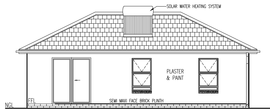
NORTH ELEVATION - 1:100
